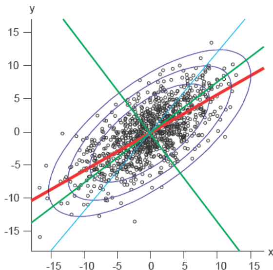
Figure 0.9 Completed Figure 0.2: Observations from N_2(0, \Sigma) ; \sigma_x = 5 , \sigma_y = 4 , \rho_{xy} = 0.7 . Regression line has the slope \hat{\beta}_1 \approx \rho_{xy}\sigma_y/\sigma_x . Also the regression line of x on y is drawn. The direction of the first major axis of the contour ellipse is determined by t_1 , the first eigenvector of \Sigma .
