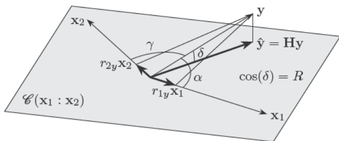
Figure 8.5 Large R^2 but r_{1y} and r_{2y} very small.
