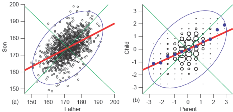
Figure 9.2 (a) Data of Pearson & Lee (1903): heights of fathers and sons, in centimeters; n = 1078 . (b) Data of Galton (1886): height of “midparent” vs. height of adult child, n = 928 . Measurements are centered and scaled so that variances are 1. The size of a circle is proportional to the number of observations in the corresponding cell of Galton’s cross-tabulation. The conditional means are marked with filled circles.
