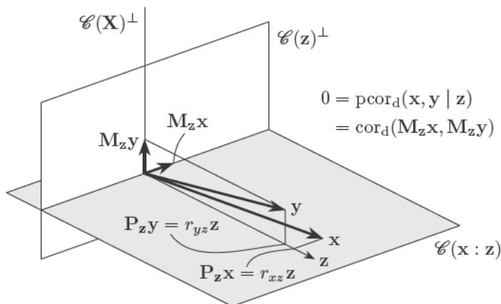
Figure 3.4 Partial correlation r_{xy.z} = 0 . Note that if y is explained by x and z , then the x 's regression coefficient is 0.
