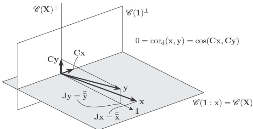
Figure 3.3 High cosine between x and y but no correlation. Vectors x and y very close to 1 .
