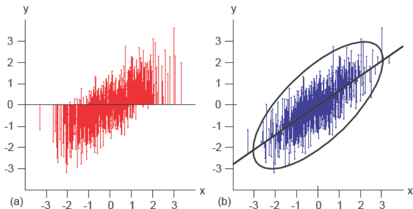
Figure 8.2 Fitting the linear model into the scatterplot of Figure 8.1. (a) Residuals from the model \mathcal{M}_0 = \{y, 1\beta_0, \sigma^2\mathbf{I}\} , (b) residuals from \mathcal{M}_{12} = \{y, 1\beta_0 + x\beta_1, \sigma^2\mathbf{I}\} .
