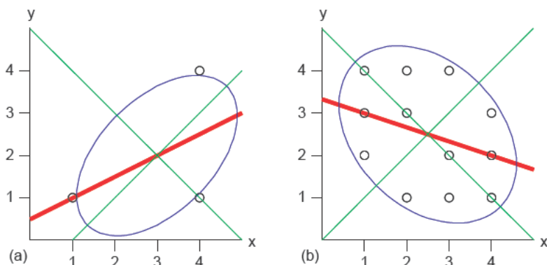
Figure 0.8 Completed Figures 0.1a and 0.1b. Regression line a bit thicker. The confidence ellipses (constant-density contours) are based on the assumption that samples are from N_2(\mu, \Sigma) , where \mu and \Sigma are equal to their sample values. The first major axis of the ellipse will be along the 135^\circ (slope -1 ) line through \mu , and it is the line satisfying the minimization Task 2 on page 1. See also Figure 19.3 (p. 404).
