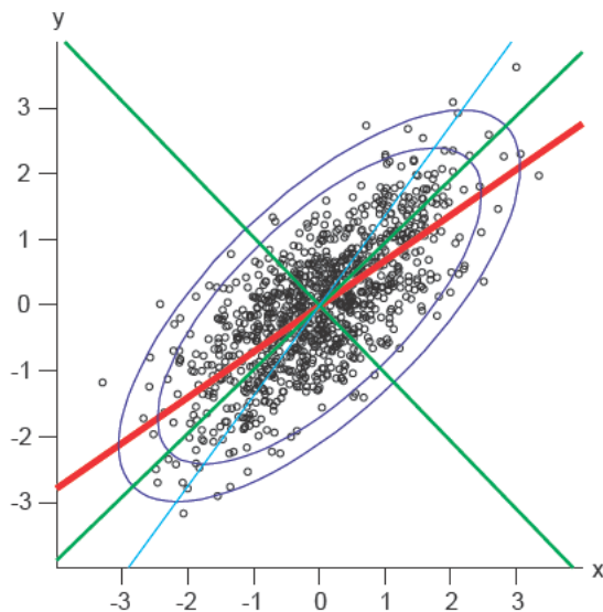
Figure 8.1 1000 observations from N_2(\mathbf{0}, \Sigma) ; \sigma_x = \sigma_y = 1 , \varrho_{xy} = 0.7 .
