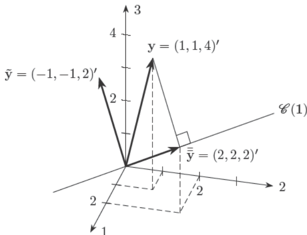
Figure 0.7 (Example 0.1) The variable vector \mathbf{y} in the variable space \mathbb{R}^3 ; \tilde{\mathbf{y}} is the centered \mathbf{y} and \bar{\bar{\mathbf{y}}} = \mathbf{J}\mathbf{y} .
