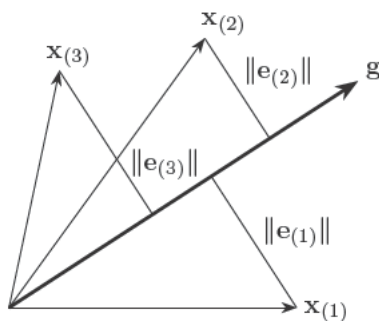
Figure 19.1 Minimizing orthogonal distances.
